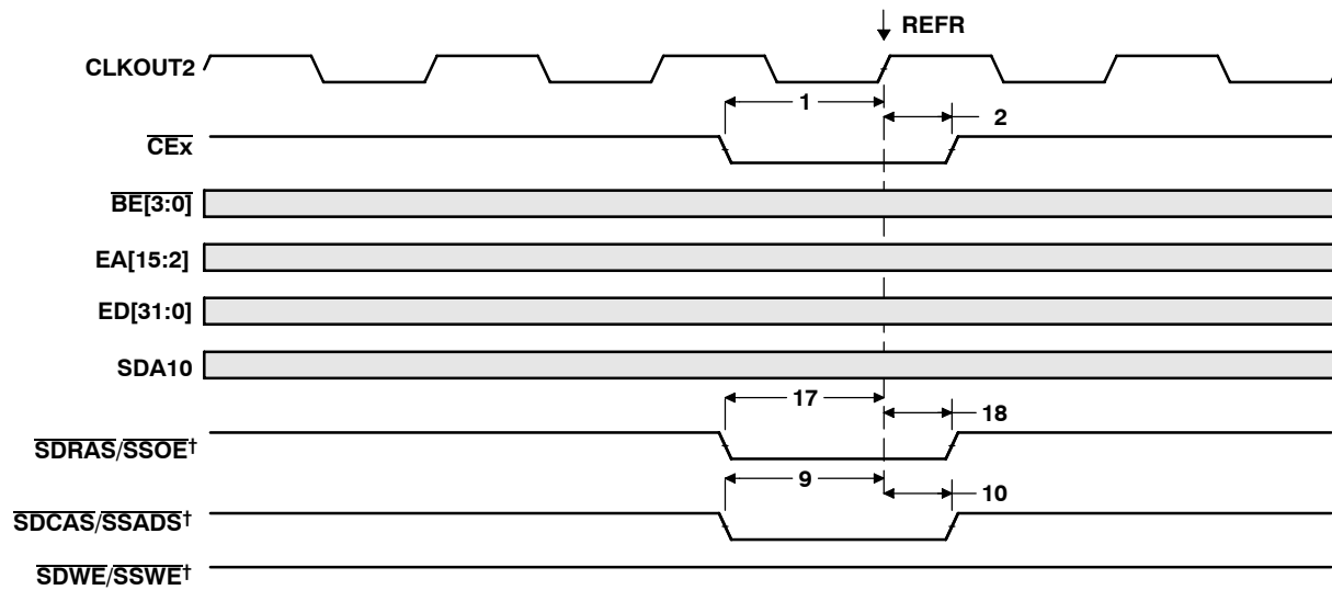
Figure 29. SDRAM REFRESH Command
